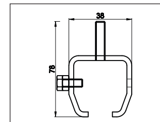
TRACK CLAMP WITH BOLT MCRT04B
