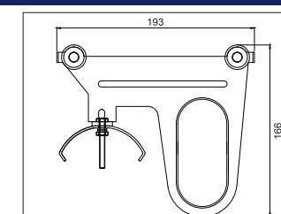
TOWING TROLLEY MCRT05
