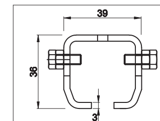
TRACK COUPLER MCRT03
