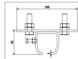
TRACK CLAMP WITH PLATE MCRT04P
