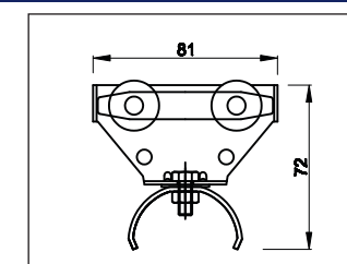
FLAT CABLE TROLLEY MCRT10A
